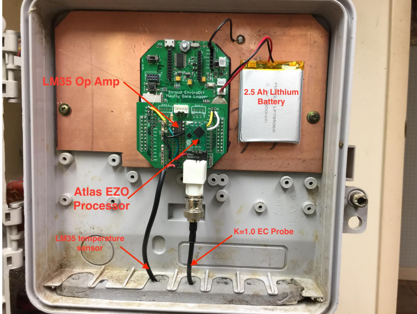
Mayfly based EC and temperature logger
